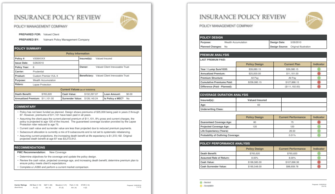
Figure 4–Policy Review Report
